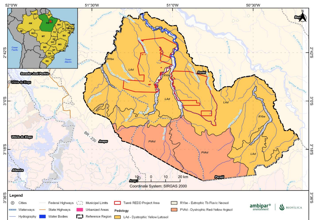
Figure 5 – Pedological characterization of the Tueré REDD+ Project.
