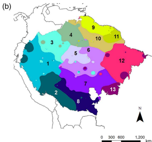
Figure 42– The floristic sub-regions of the Amazon described by Silva-Souza and Souza (2020): corresponds to the authors' Figure 2b. Source: Silva-Souza and Souza (2020) 136 .
