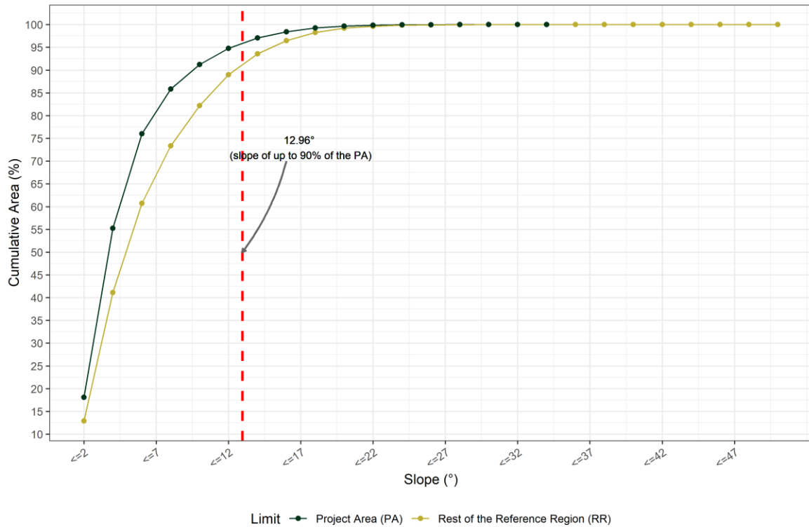
Figure 23 – Slope distribution in the Project Area and the Rest of the Reference Region.
