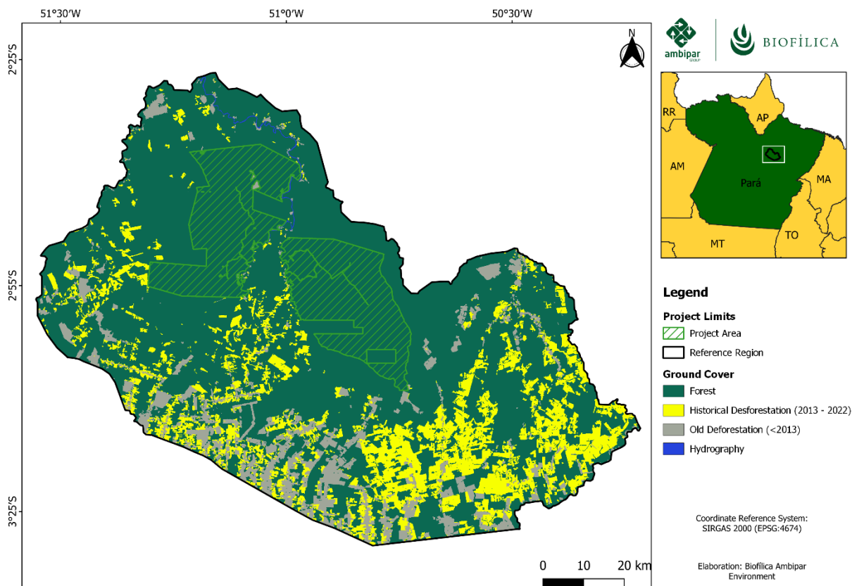
Figure 25 – Map of forest coverage in August 26, 2022.
