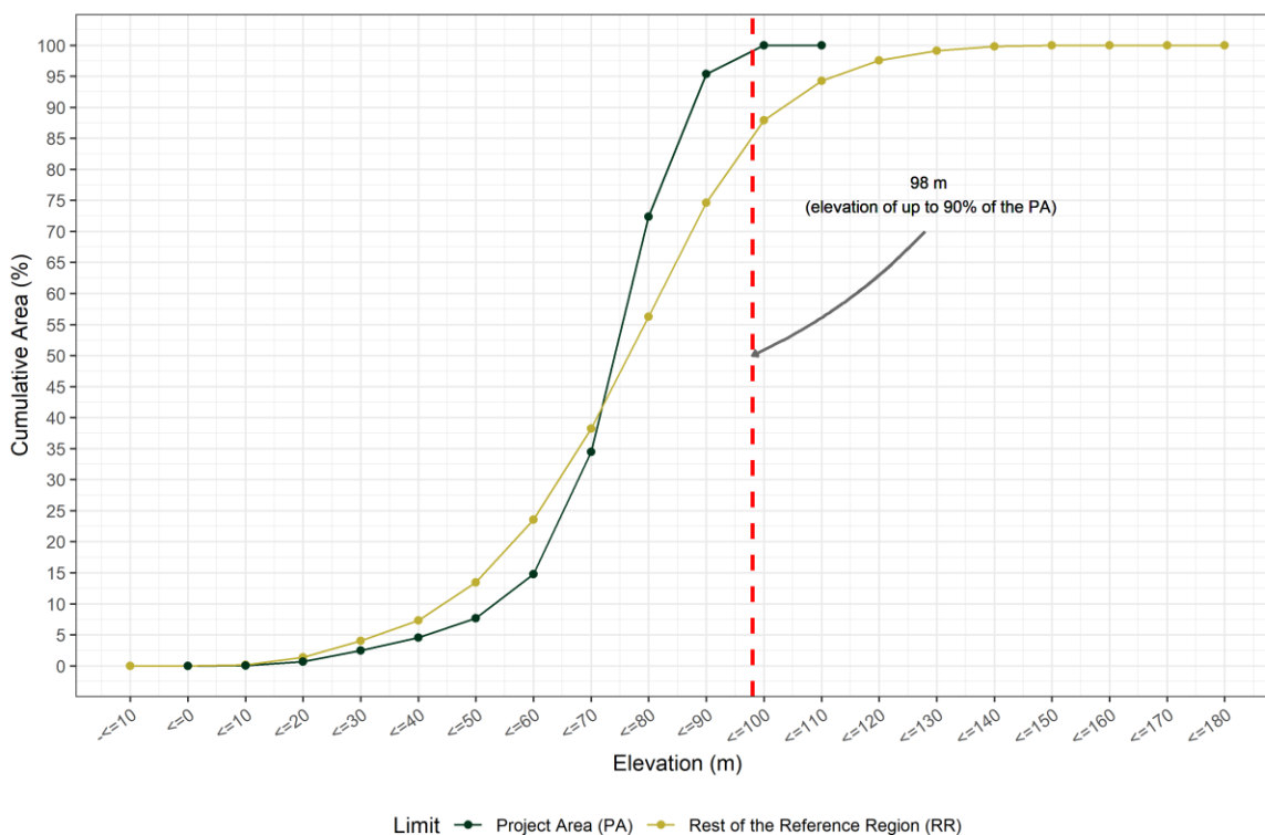
Figure 22 – Elevation distribution in the Project Area and the Rest of the Reference Region.
